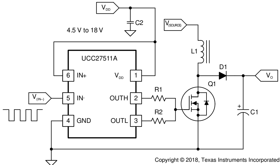
图 6-5. Using Inverting Input (IN+ Is Tied To V DD Enable Output)
