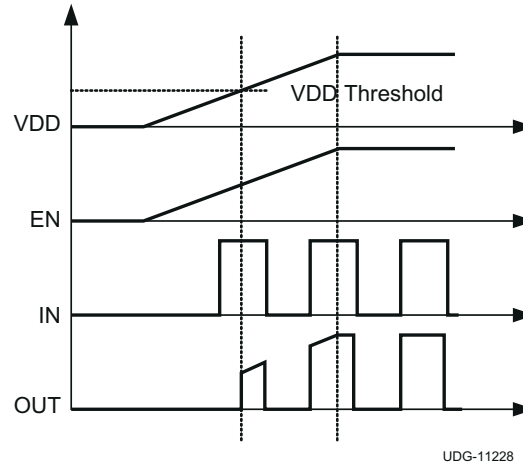
图 8-2. Power-Up Sequence
