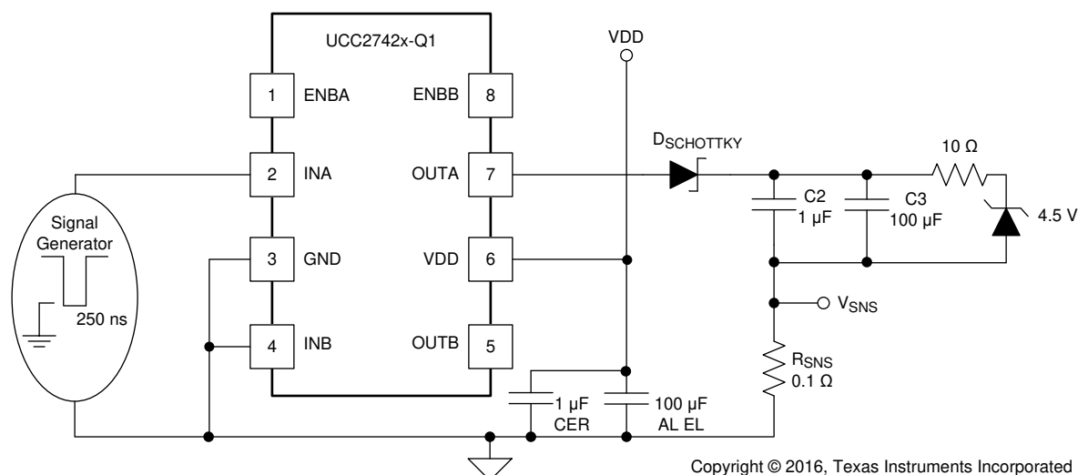
图 8-3. Current Source Capability Test
