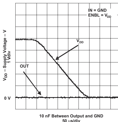
图 7-24. Output Behavior vs VDD (Noninverting)
