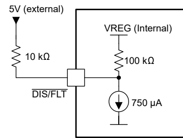
图 8-17. External Pullup for 5-V Supply
