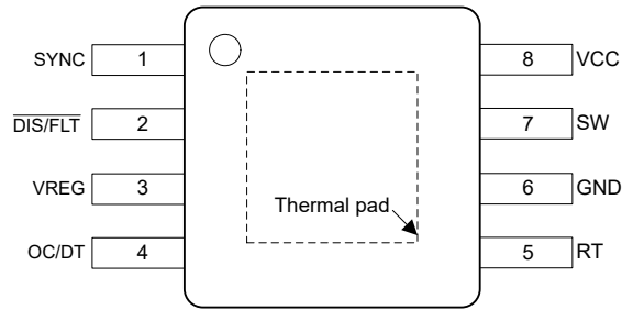
图 6-1. DGN Package, 8-Pin PDSO (Top View)
