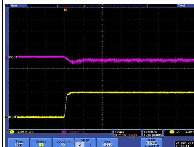
Transient Response
