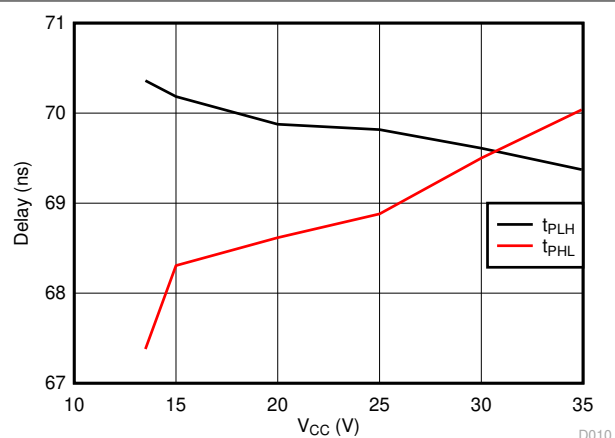
图 6-11. Propagation delay versus Supply voltage
