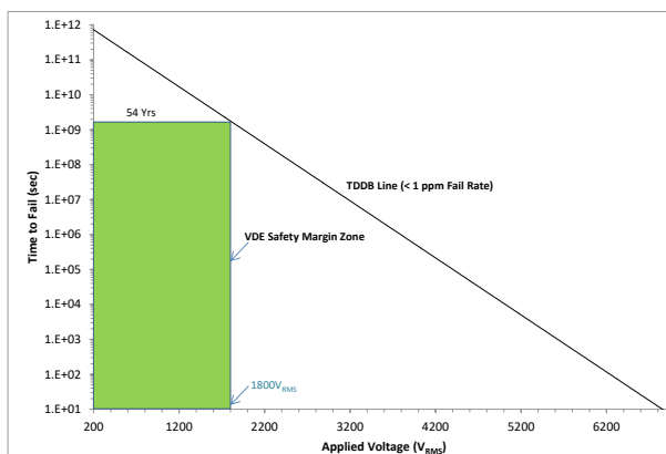
图 6-1. Reinforced Isolation Capacitor Life Time Projection
