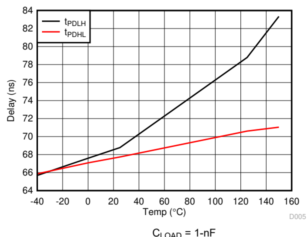
图 6-8. Propagation delay versus Temperature
