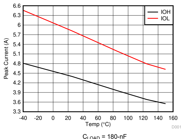
图 6-4. Output Drive currents versus Temperature
