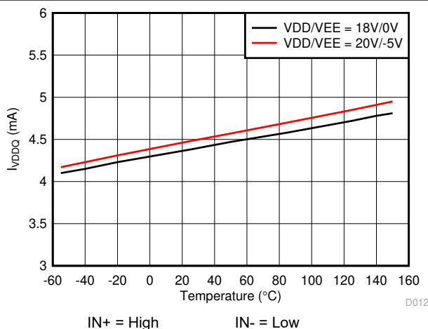
图 5-8. I_{VDDQ} Supply Current vs Temperature
