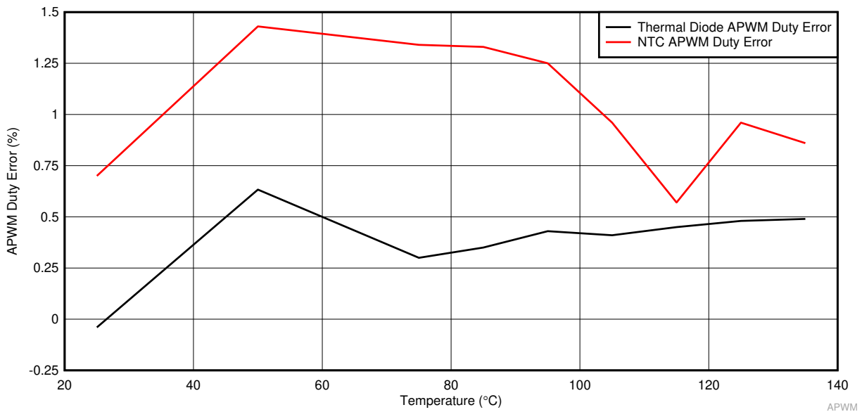
图 8-10. APWM Duty Error Without Calibration
