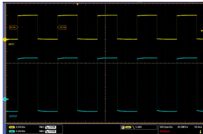
图 8-14. PWM Input (yellow) and Driver Output (blue)
