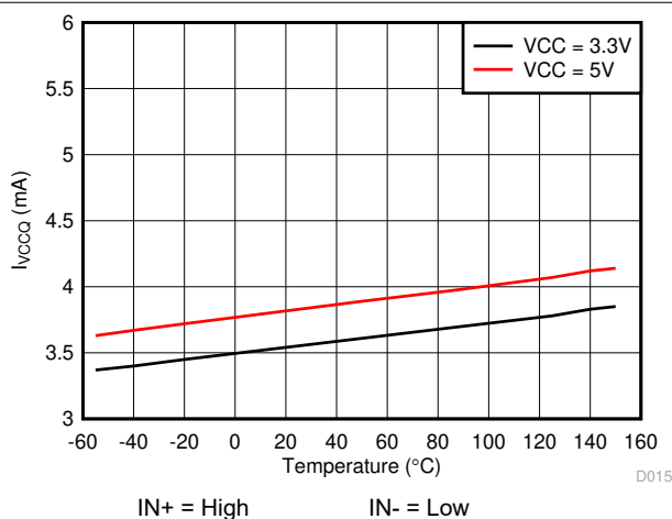
图 5-5. I_{VCCQ} Supply Current vs Temperature
