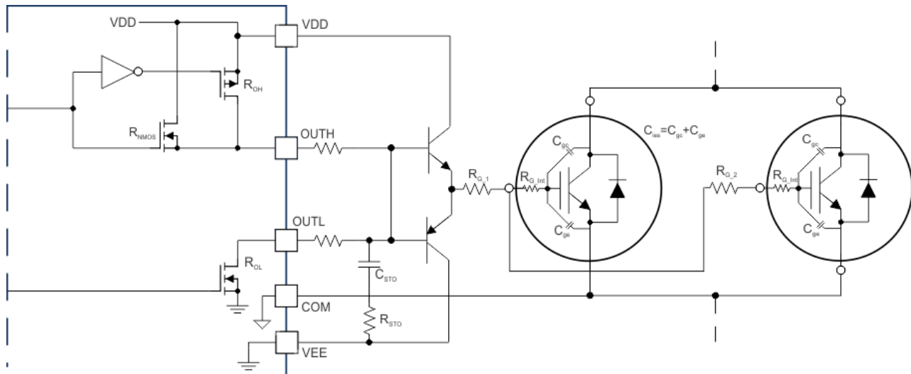
图 8-13. Current Buffer for Increased Drive Strength
