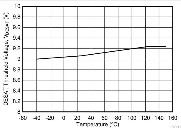
图 5-23. V_{DESAT} DESAT Threshold Voltage vs Temperature
