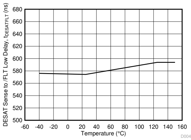
图 5-26. t_{DESATFLT} DESAT Sense to /FLT Low Delay Time vs Temperature
