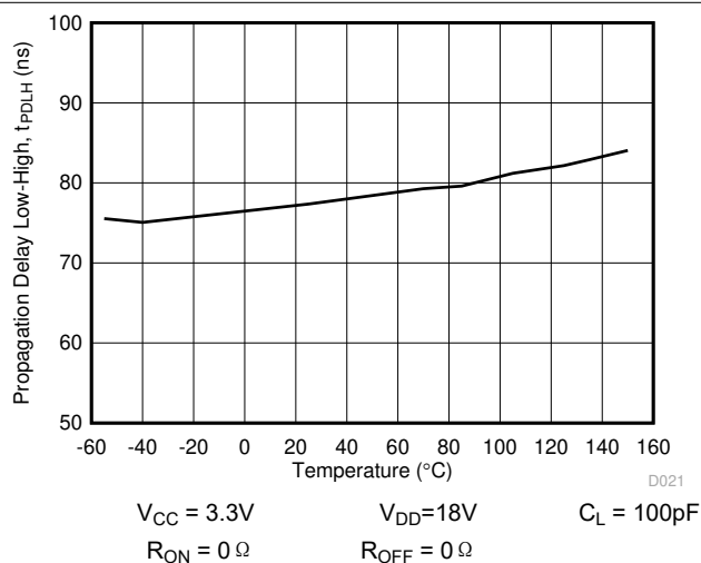
图 5-13. Propagation Delay t_{PDLH} vs Temperature
