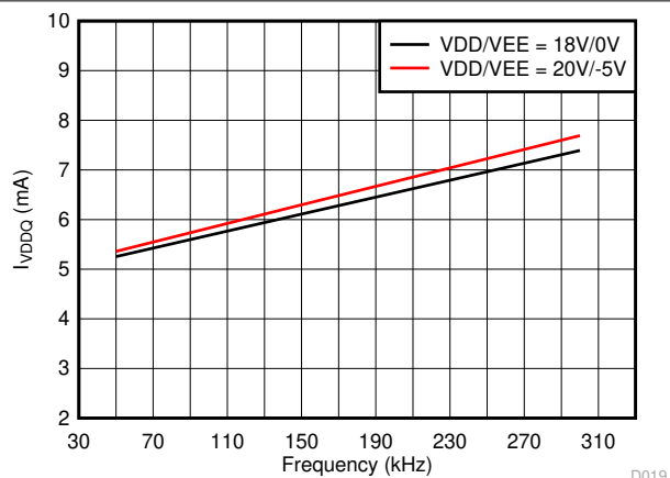
图 5-10. I_{VDDQ} Supply Current vs Input Frequency
