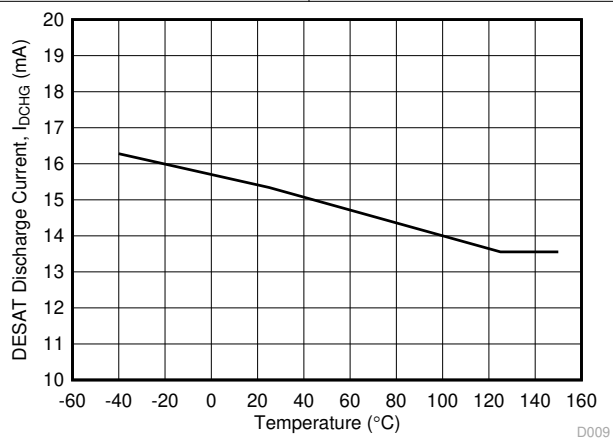
图 5-29. I_{\text{DCHG}} DESAT Discharge Current vs Temperature
