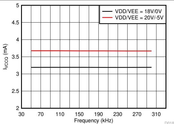
图 5-7. I_{VCCQ} Supply Current vs Input Frequency
