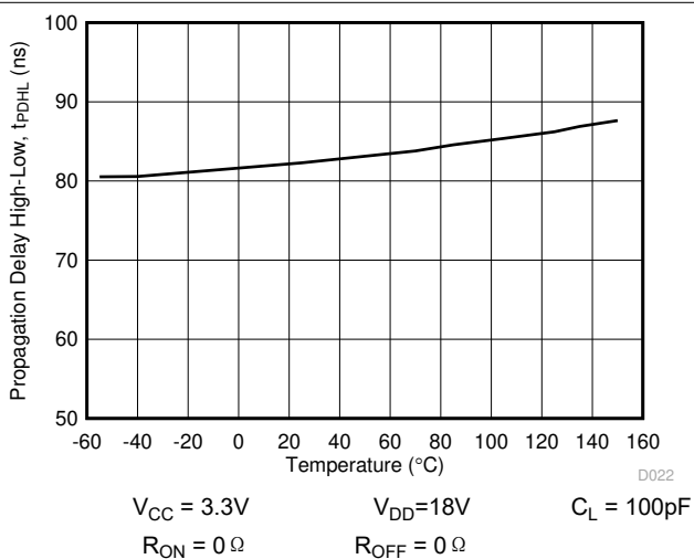
图 5-14. Propagation Delay t_{PDHL} vs Temperature
