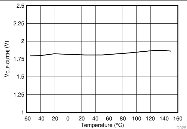
图 5-18. V_{CLP-OUT(H)} Short Circuit Clamping Voltage vs Temperature
