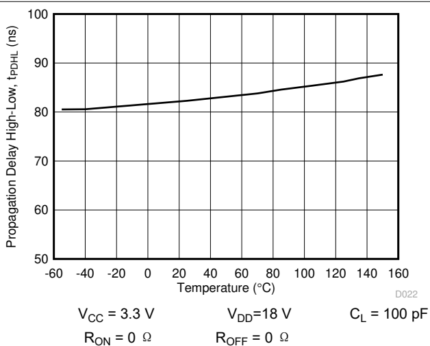
图 6-15. Propagation Delay t_{PDHL} vs Temperature
