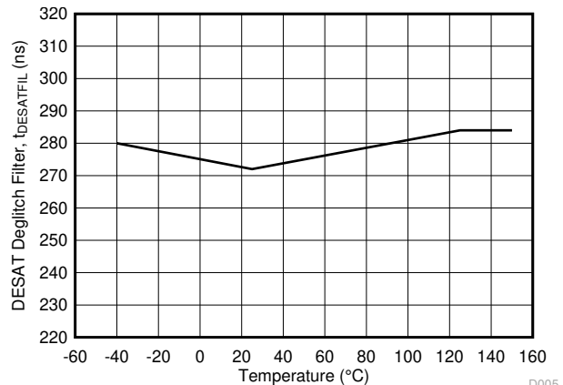
图 6-27. t_{DESATFIL} DESAT Deglitch Filter vs Temperature
