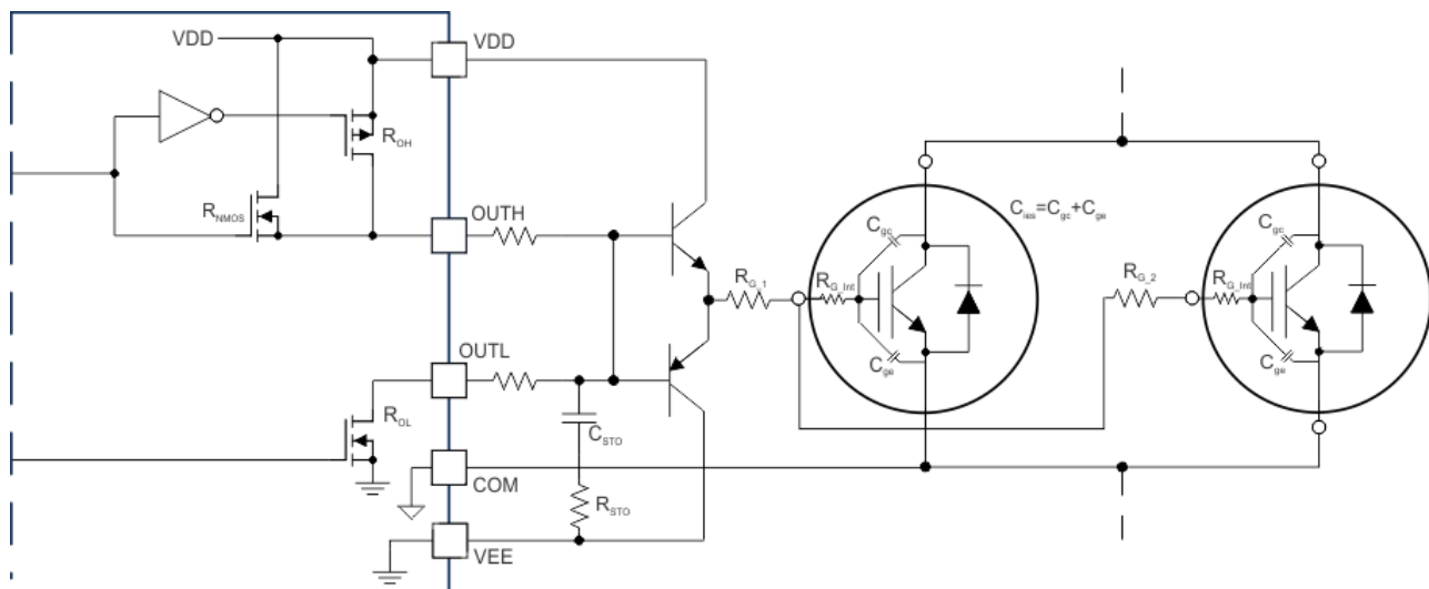
图 9-13. Current Buffer for Increased Drive Strength
