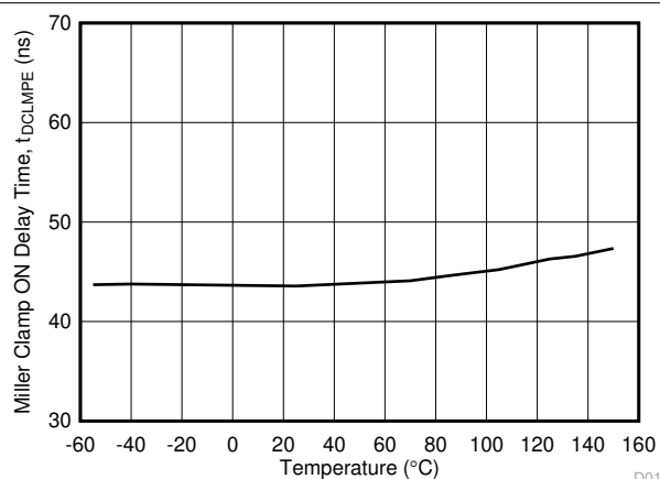
图 6-23. t_DCLMPE Miller Clamp ON Delay Time vs Temperature
