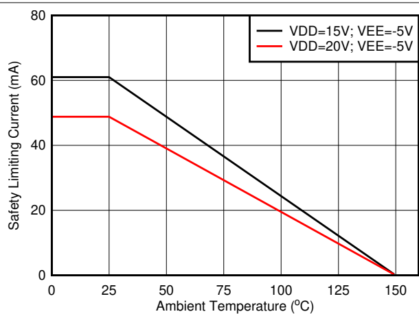
图 6-1. Thermal Derating Curve for Limiting Current per VDE
