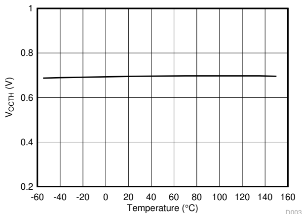
图 6-24. V_{OCTH} OC Detection Threshold vs Temperature
