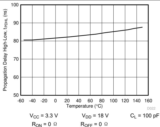
图 6-15. Propagation Delay t_{PDLH} vs Temperature
