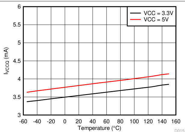
图 6-6. I_{VCCQ} Supply Current vs Temperature
