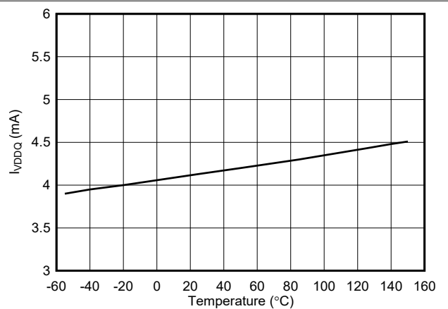
图 6-10. I_{VDDQ} Supply Current vs Temperature
