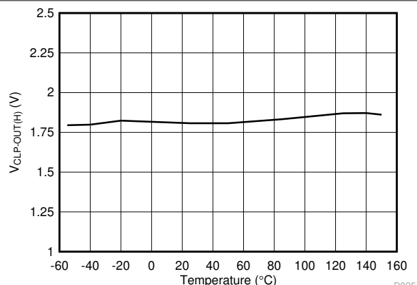
图 6-19. V_CLP-OUT(H) Short Circuit Clamping Voltage vs Temperature
