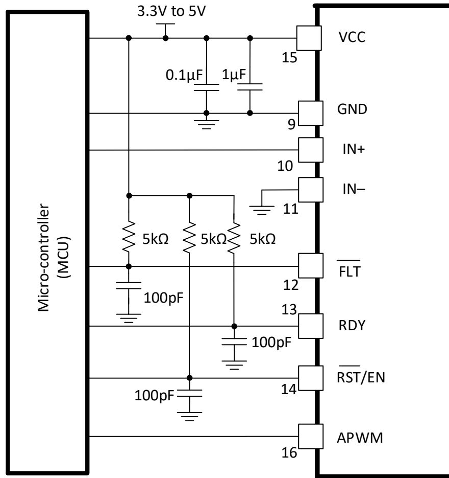
图 9-3. FLT, RDY and RST/EN Pins Circuitry
