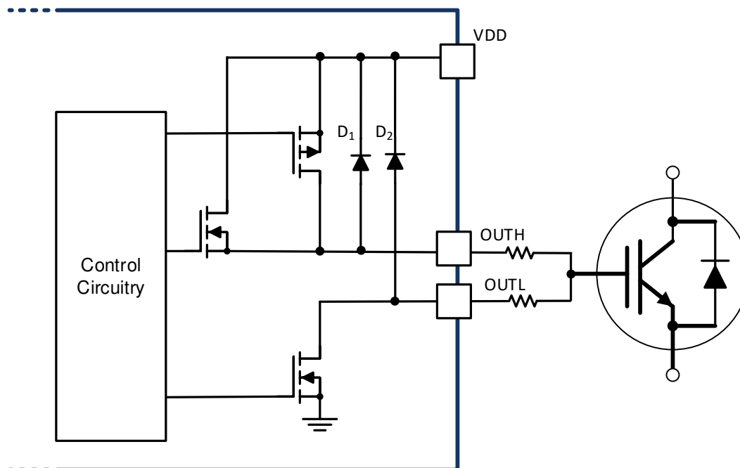
图 8-3. Short Circuit Clamping
