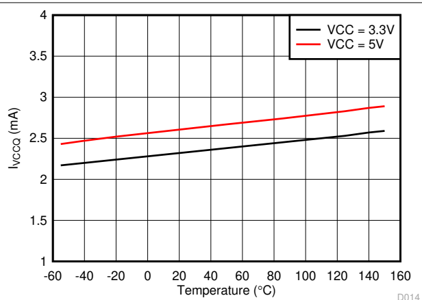
图 6-7. I_{VCCQ} Supply Current vs Temperature
