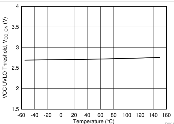
图 5-13. VCC UVLO vs. Temperature
