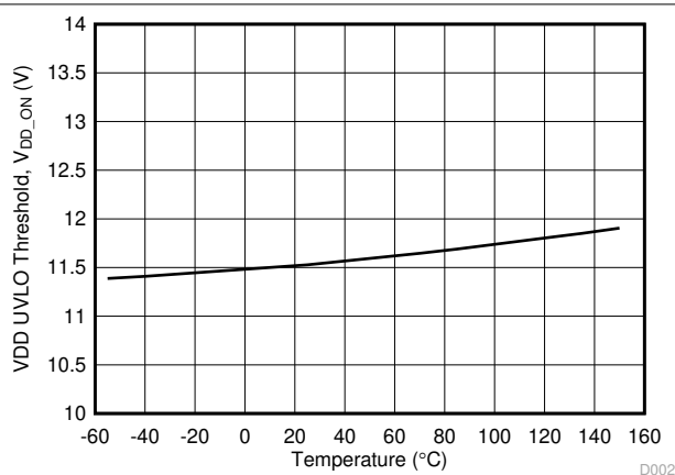
图 5-12. VDD UVLO vs. Temperature
