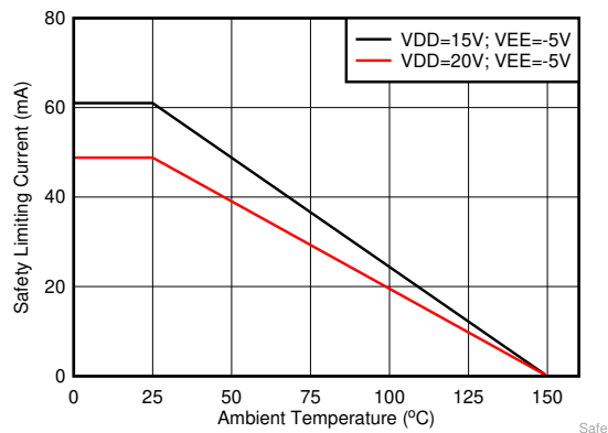
图 5-2. Thermal Derating Curve for Limiting Current per VDE
