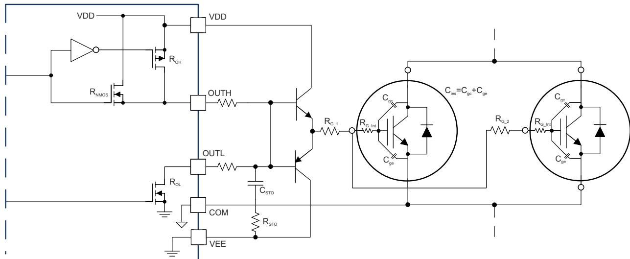
图 8-16. Current Buffer for Increased Drive Strength
