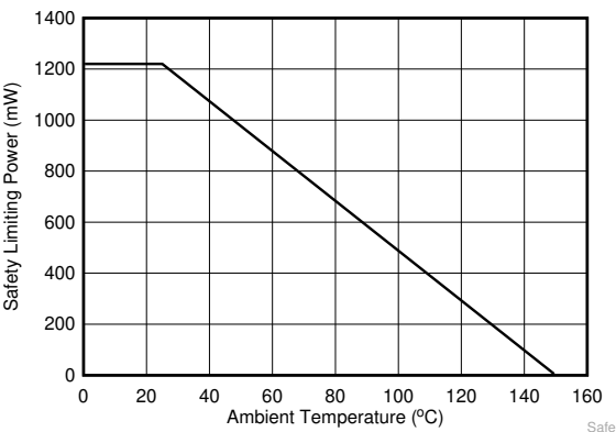
图 5-3. Thermal Derating Curve for Limiting Power per VDE
