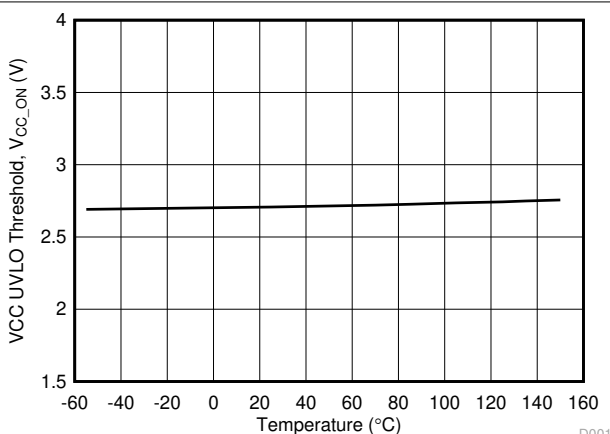
图 5-13. VCC UVLO vs. Temperature
