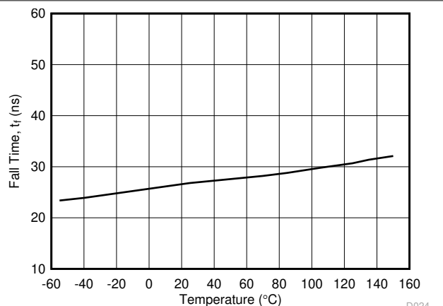
图 5-17. t_f Fall Time vs. Temperature
