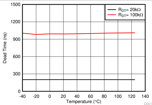
图 6-29. Dead Time vs. Temperature (with R_{DT} = 20 k \Omega and 100 k \Omega )
