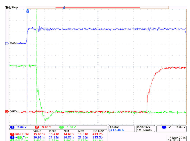
图 9-6. Zoomed-In bench-test waveform
