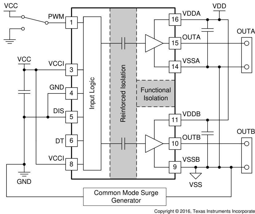
图 7-5. Simplified CMTI Testing Setup
