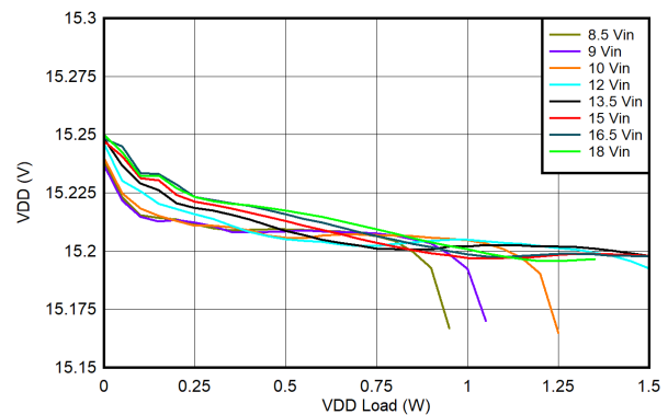
图 6-29. UCC14341B-Q1 V_{VDD-VEE} 负载调节: T_{AMBIENT} = 85^{\circ}C , V_{VDD-VEE} = 15V , V_{COM-VEE} = 4V
