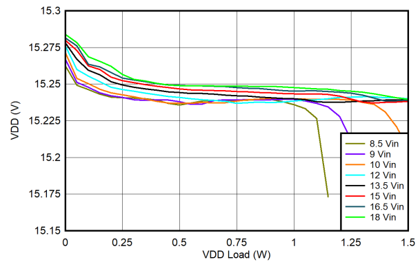
图 6-27. UCC14341B-Q1 V_{VDD-VEE} 负载调节: T_{AMBIENT} = -40^{\circ}C , V_{VDD-VEE} = 15V , V_{COM-VEE} = 4V
