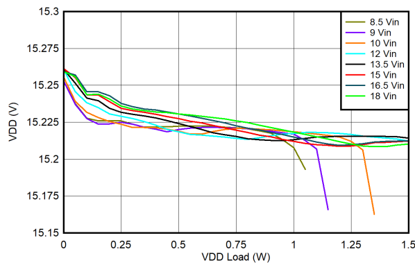
图 6-28. UCC14341B-Q1 V_{VDD-VEE} 负载调节: T_{AMBIENT} = 25^{\circ}C , V_{VDD-VEE} = 15V , V_{COM-VEE} = 4V
