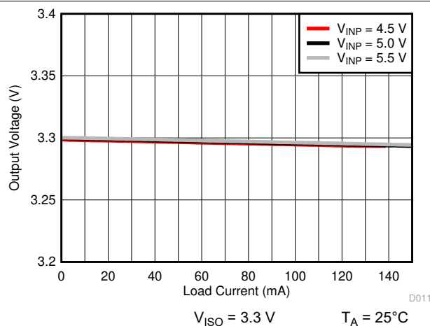
图 6-18. Isolated Supply Voltage ( V_{ISO} ) vs Load Current ( I_{ISO} )
