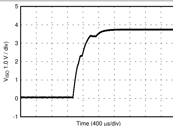
图 8-23. V_{ISO} Soft Start at 90% Rated Load, 5.0-V Input, 3.7-V Output
