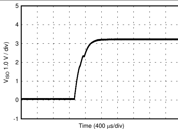
图 8-25. V_{ISO} Soft Start at 90% Rated Load, 5.0-V Input, 3.3-V Output
