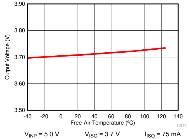
图 6-23. Isolated Supply Voltage ( V_{ISO} ) vs Free-Air Temperature
