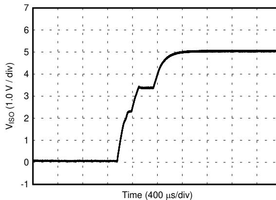
图 8-21. V_{ISO} Soft Start at 90% Rated Load, 5.0-V Input, 5.0-V Output
