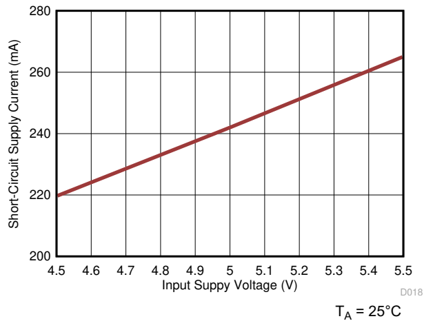
图 6-24. Short-Circuit Supply Current ( I_{IN\_SC} ) vs Supply Voltage ( V_{INP} )
