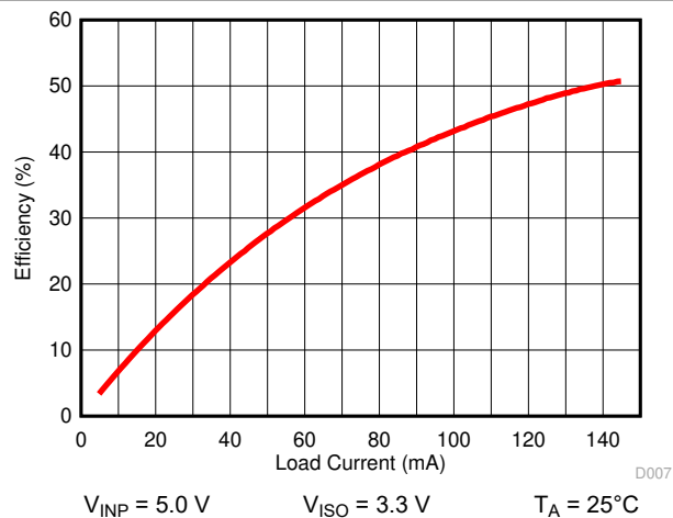
图 6-14. Power Supply Efficiency vs Load Current ( I_{ISO} )
