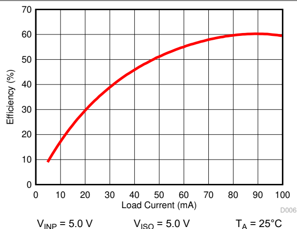
图 6-12. Power Supply Efficiency vs Load Current ( I_{ISO} )
