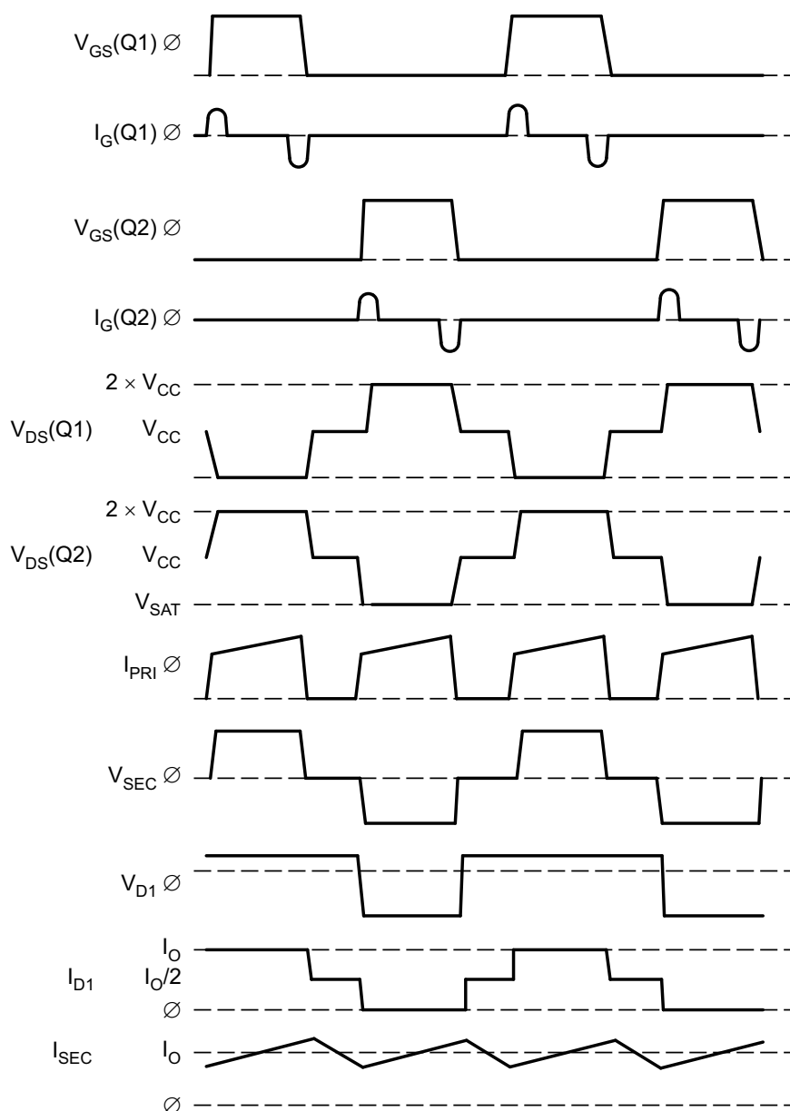
图 8-5. Basic Push-Pull Waveforms
