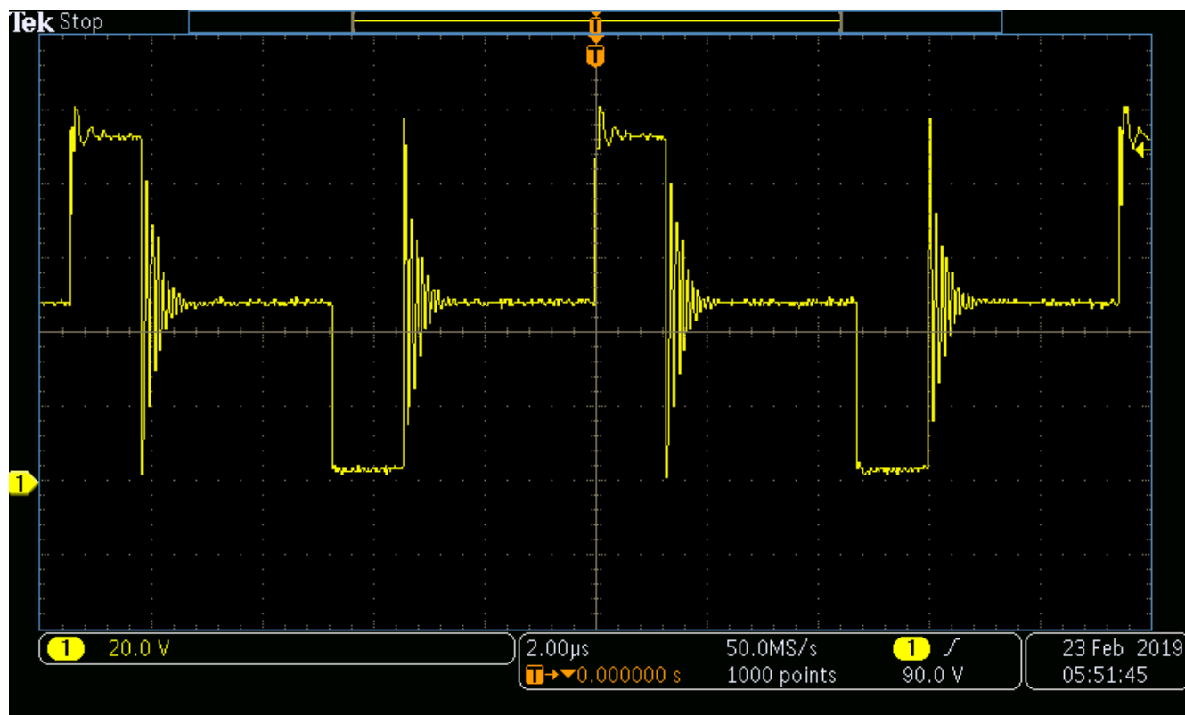
图 8-6. Voltage Stress Across Main Switching MOSFETS Q1 and Q2
