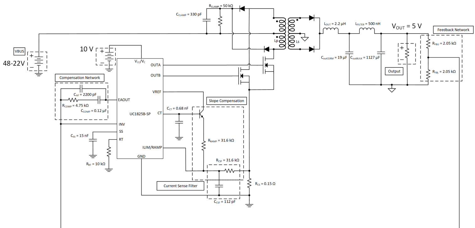
图 8-4. Typical Application
