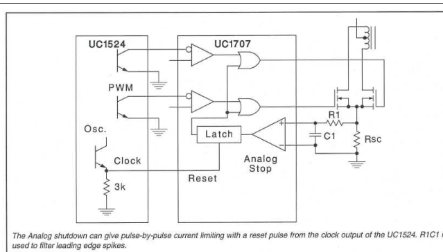
Figure 6. Current Limiting
