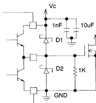
Figure 13. Power MOSFET Drive Circuit
