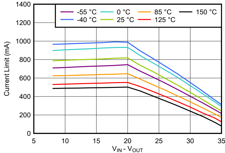
图 6-1. Current-Limit vs V_{\text{Head-room}} Behavior (New Chip)
