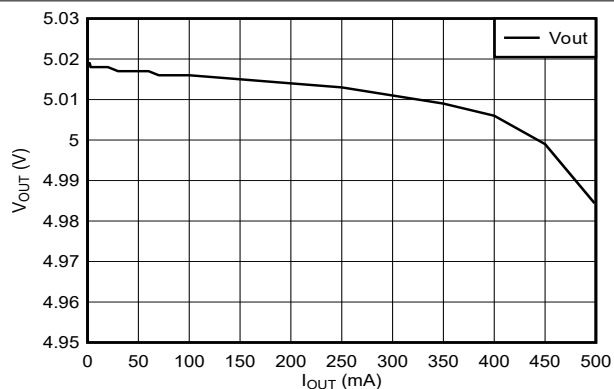
图 5-2. Load Regulation at T_J = 25^\circ\text{C} (New Chip)
