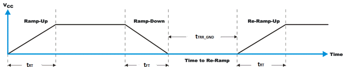
Figure 8-3. V_{CC} is lowered to 0V and then ramped up
