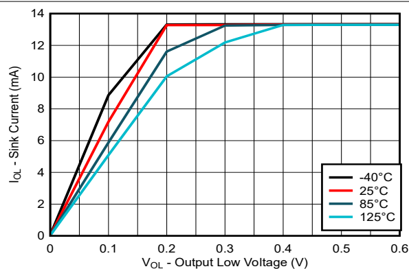
Figure 5-6. I/O Sink Current vs Output Low Voltage for Different Temperature ( T_A ) for V_{\text{CC}} = 3.3\text{V}
