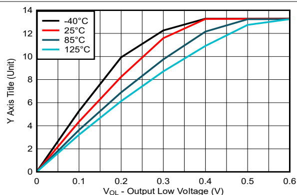
Figure 5-4. I/O Sink Current vs Output Low Voltage for Different Temperature ( T_A ) for V_{\text{CC}} = 1.8\text{V}
