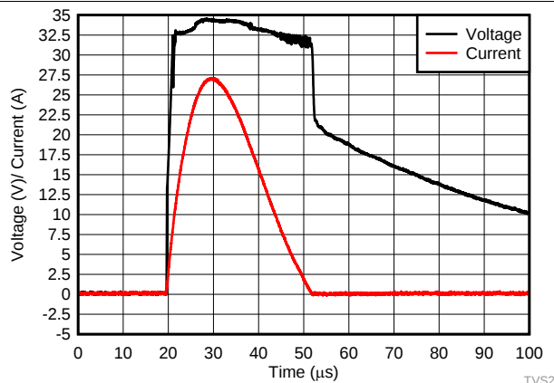
图 1. 8/20 \mu s Surge Response at 27 A
