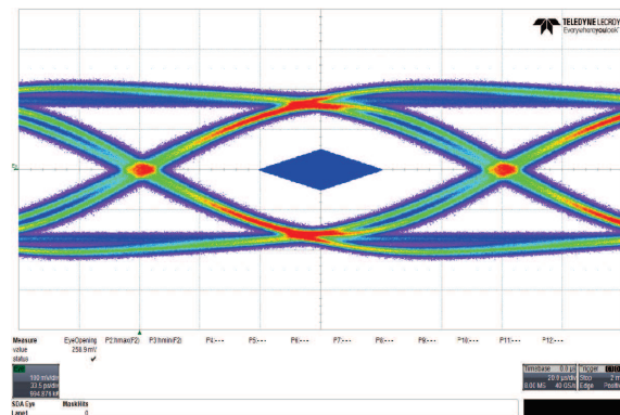
Figure 37. Downstream Port 1
