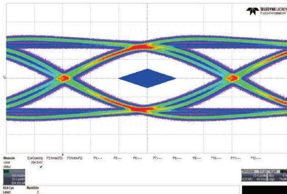
Figure 36. Upstream Port
