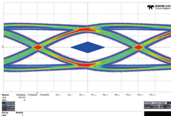
Figure 38. Downstream Port 2
