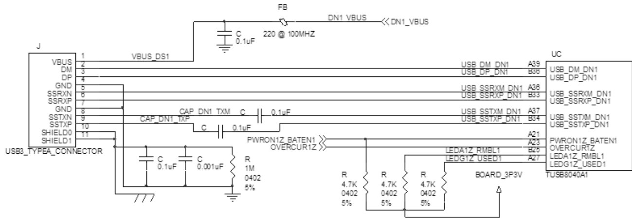
图 8-5. Downstream Port 3 Implementation
