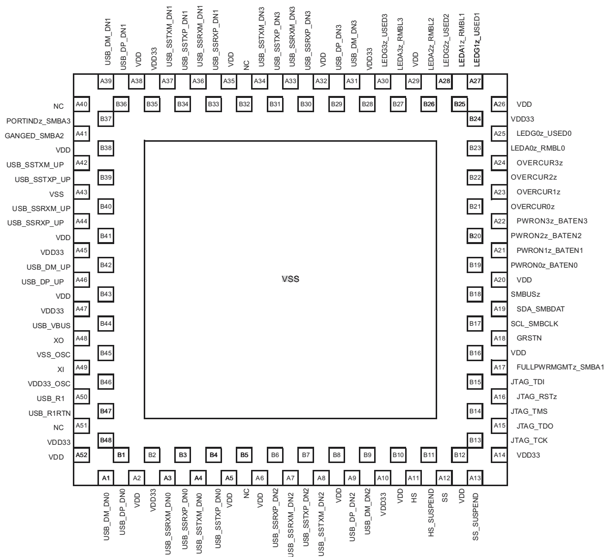
图 5-1. 100-Pin TUSB8040A1 RKM Package, 100-Pin WQFN (Top View)
