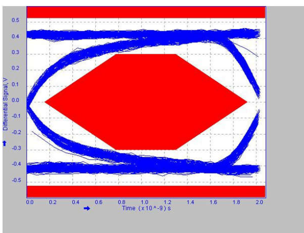
图 8-19. High-Speed Downstream Port 4
