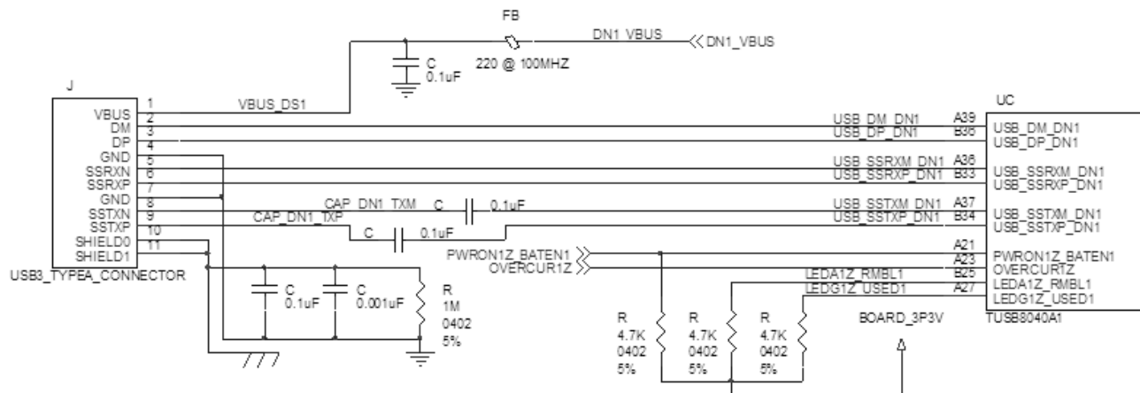
图 8-4. Downstream Port 2 Implementation
