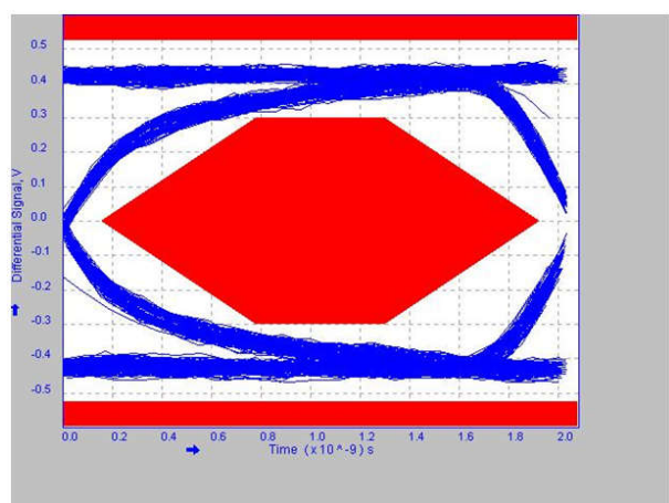
图 8-18. High-Speed Downstream Port 3
