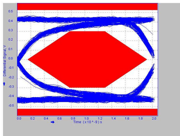
图 8-17. High-Speed Downstream Port 2
