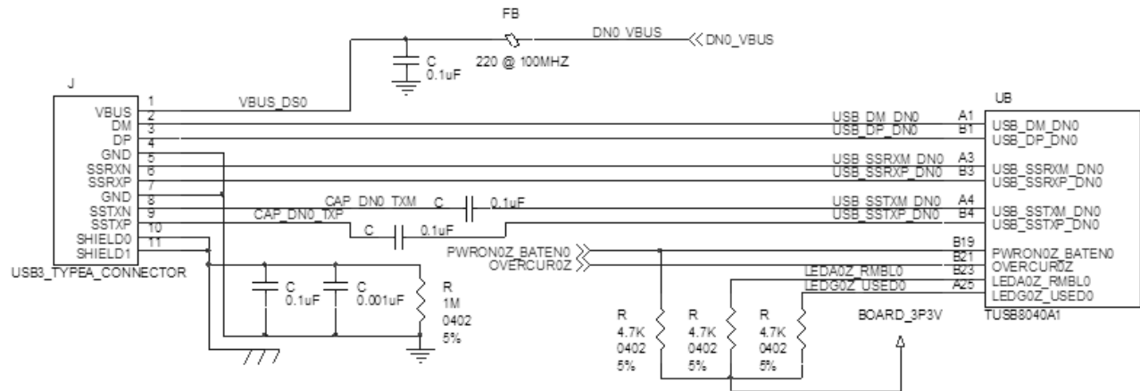
图 8-3. Downstream Port 1 Implementation
