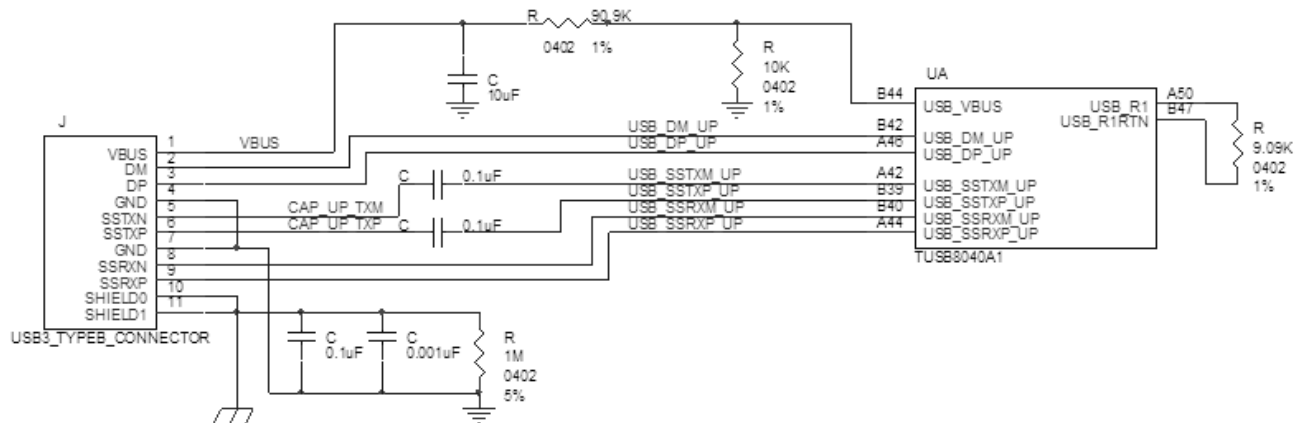
图 8-2. Upstream Port Implementation
