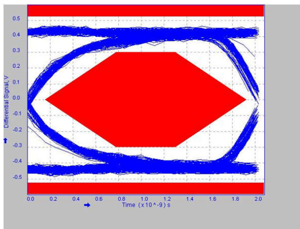
图 8-15. High-Speed Upstream Port
