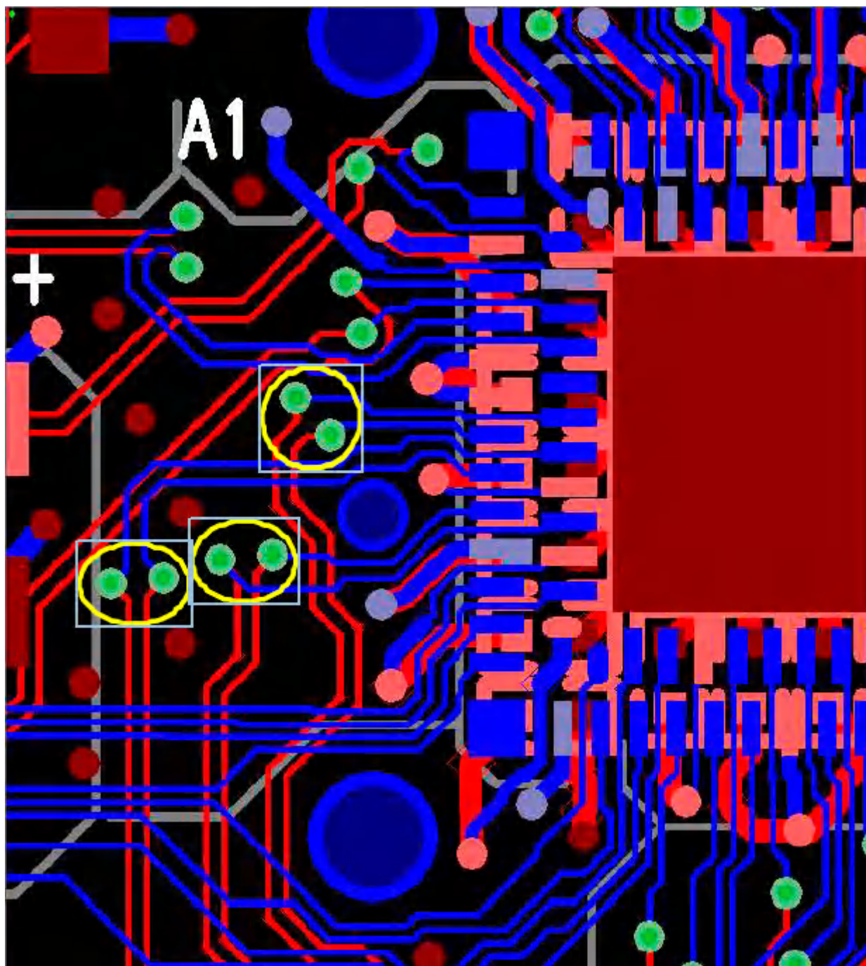
图 8-20. Using Via Placement to Cross the SSTX and SSRX Pairs
