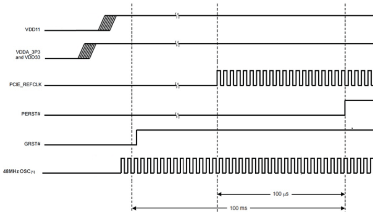
图 7-16. Power-Up Sequence
