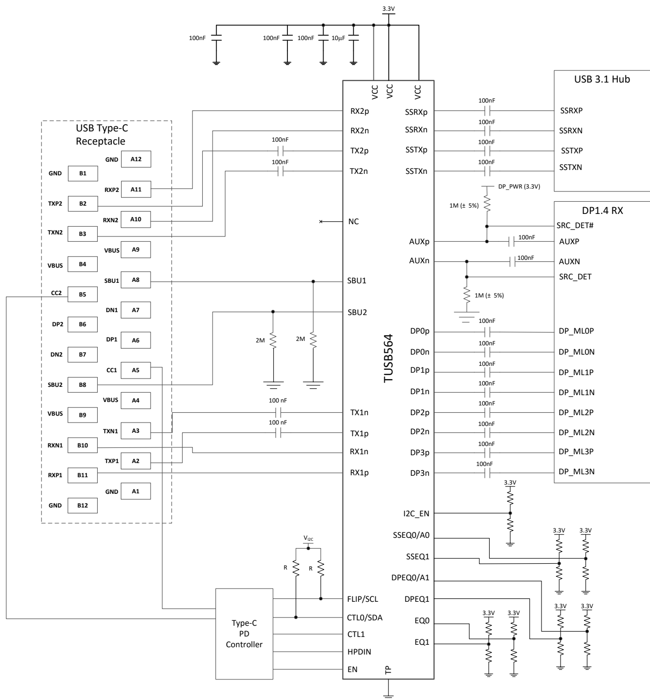
图 9-2. Application Circuit
