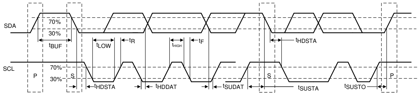
图 7-1. I²C Timing Diagram Definitions
