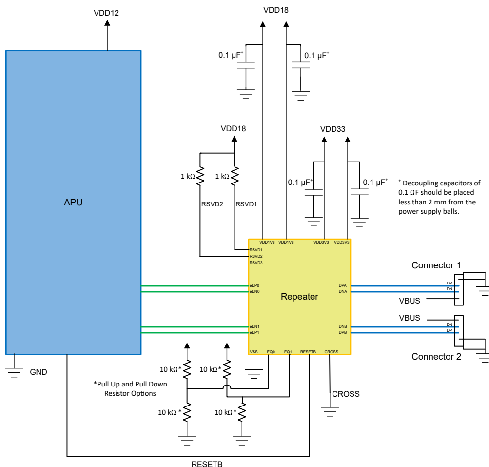
图 8-1. Typical Dual Port System Implementation
