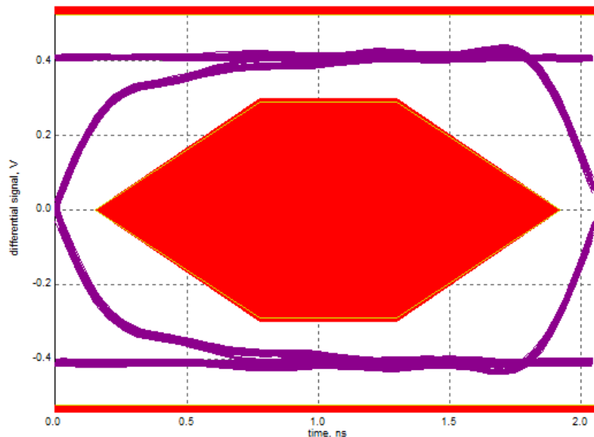
图 8-2. Typical USB 2.0 High Speed Eye Diagram
