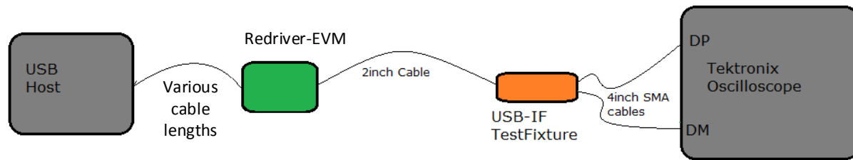
图 8-2. Near End Eye Measurement Set-Up With Pre-Channel Cable
