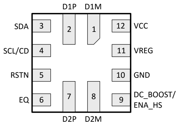
Pin Functions
