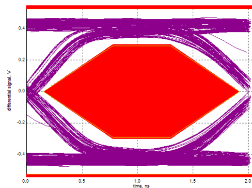
图 5. USB2.0 HS Eye diagram, Host far-end with 5m cable pre-channel loss with TUSB213-Q1
