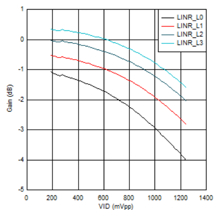
图 4-8. USB CTX1 VOD Linearity Settings at 5 GHz and EQ = 0
