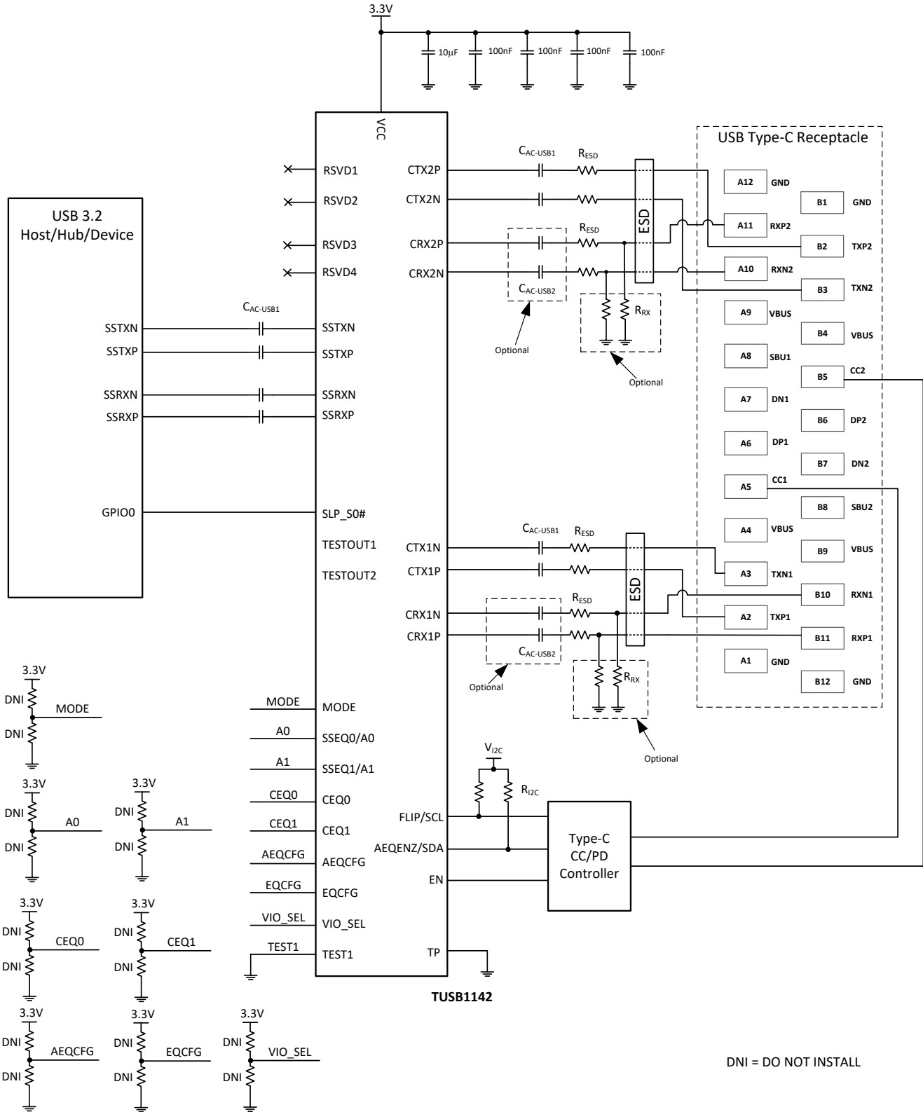
图 7-2. Application Circuit
