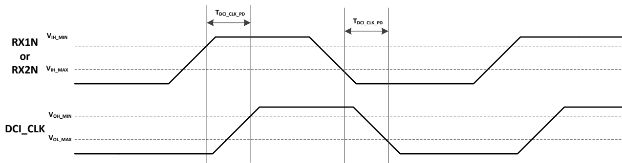
图 13. DCI Clock Propagation Delay
