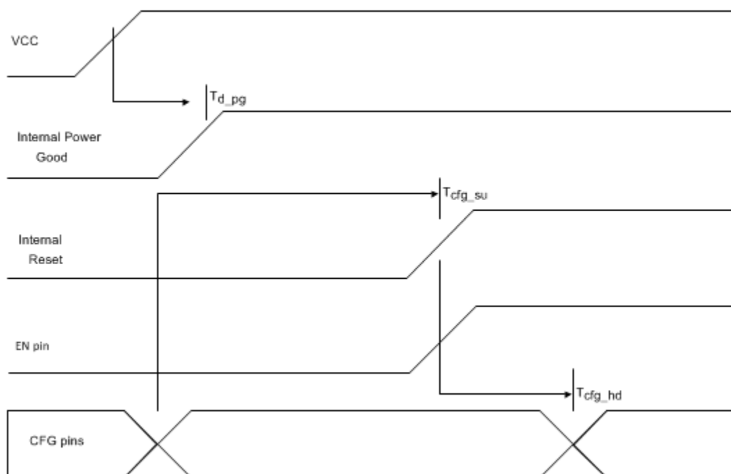
图 5-2. Power-Up Diagram
