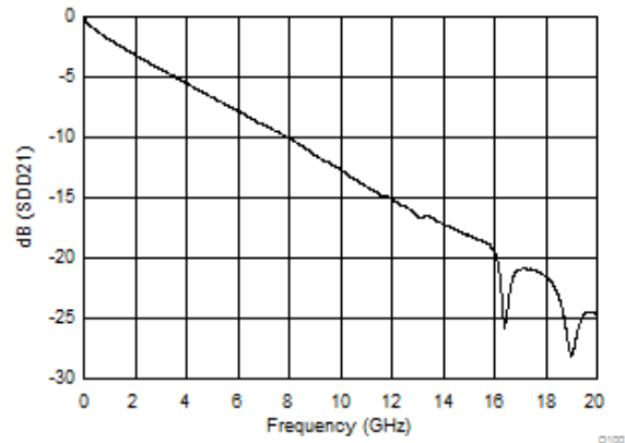
图 7-3. Insertion Loss for 8-inch 4mil FR4 Trace
