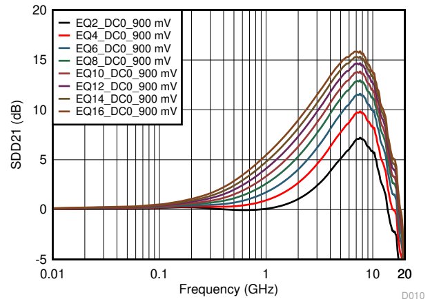
图 5-10. 900mV DC0 Gain Even EQ Settings Curves
