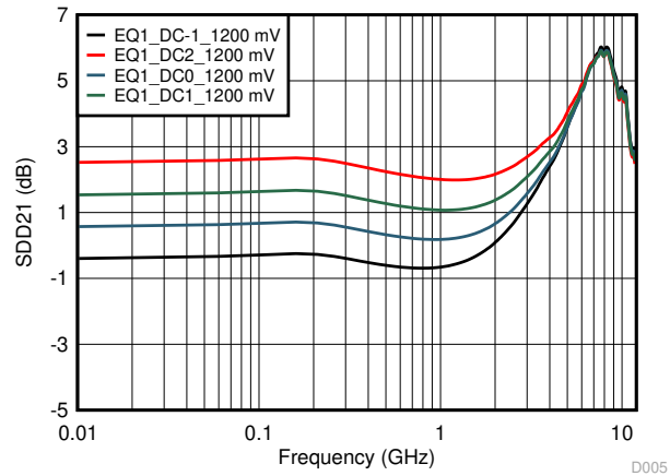
图 5-5. 1200mV DC Gain Adjustments Curves
