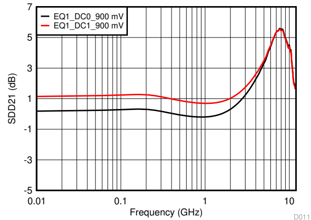
图 5-11. 900mV DC Gain Adjustment Curves
