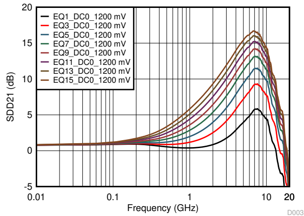
图 5-3. 1200mV DC0 Gain Odd EQ Settings Curves
