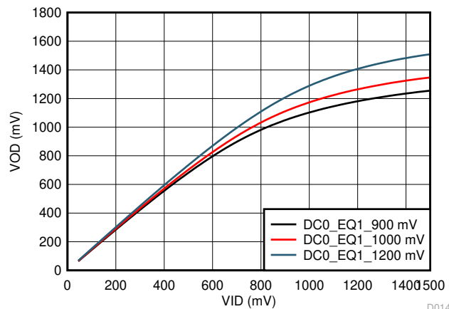
图 5-14. 5GHz Sine Wave VID vs VOD Linearity Range Setting
