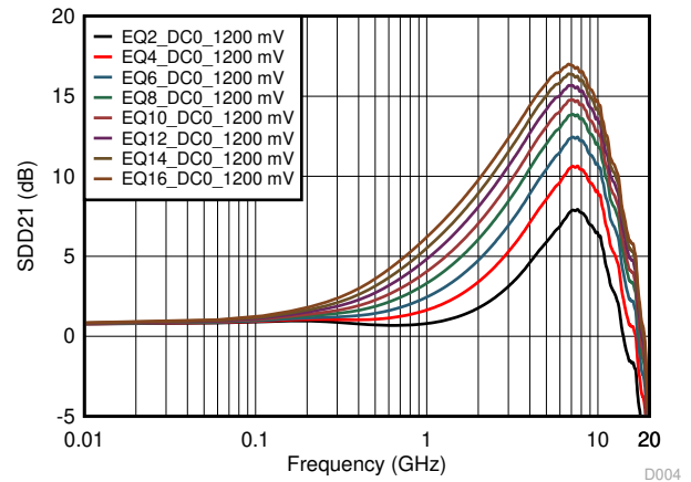
图 5-4. 1200mV DC0 Even EQ Settings Curves
