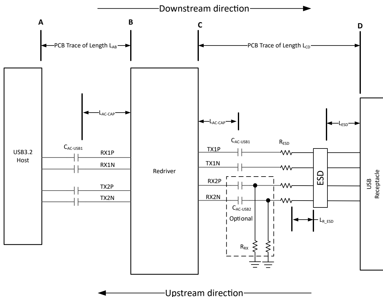
图 7-1. TUSB1002A in USB3.2 x1 Host Application
