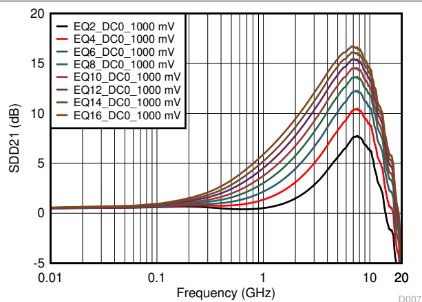
图 5-7. 1000mV DC0 Gain Even EQ Settings Curves
