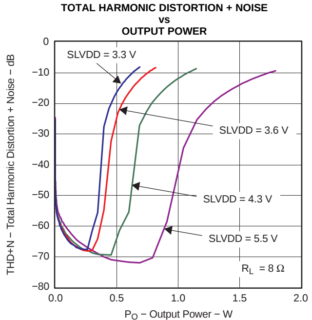
Figure 4-10. Class-D Speaker-Driver Output Power ( R_L = 8 \Omega , SLVDD = 3.3 V to 5.5V, Driver Gain = 18 dB)
