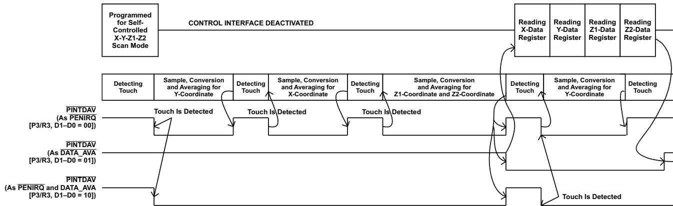
Figure 5-49. TSC2117 Self-Controlled X-Y-Z1-Z2 Scan Mode
