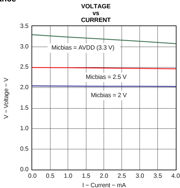
Figure 4-13. Micbias
