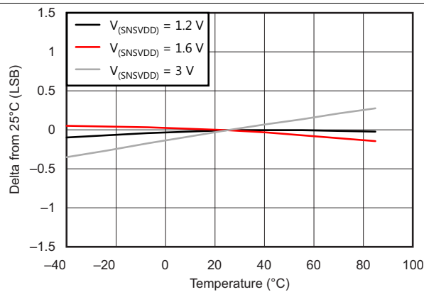
图 3. Change in Offset vs Temperature
