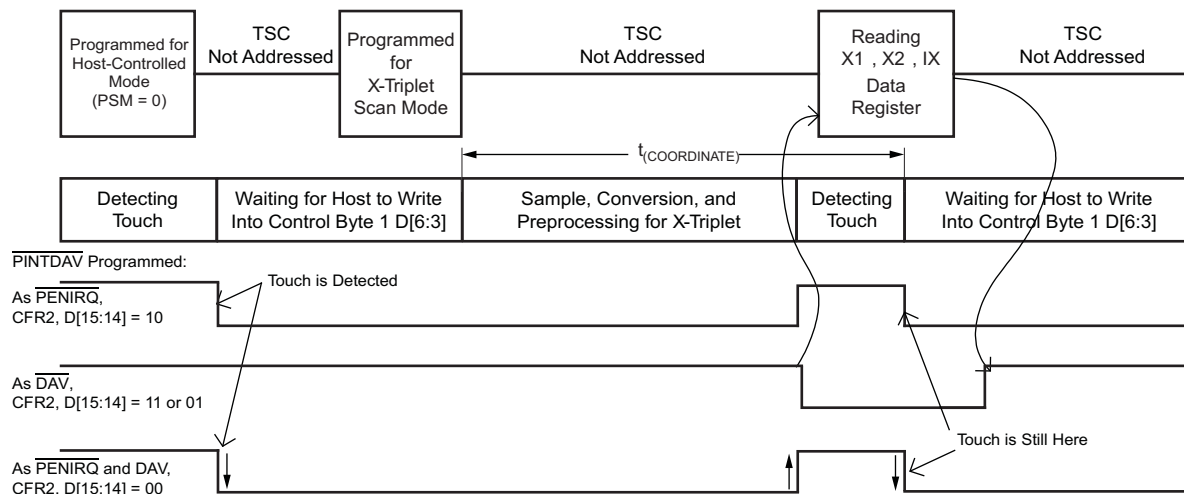
图 28. Example of a Single X-Triple Touch-Screen Scan (With Panel Stabilization Time) Using TSMODE 3
