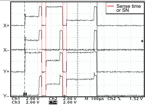
图 54. Panel Voltage Stabilization 0 \mu s, 100 \mu s, and 500 \mu s
