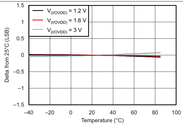
图 4. Change in Gain vs Temperature
