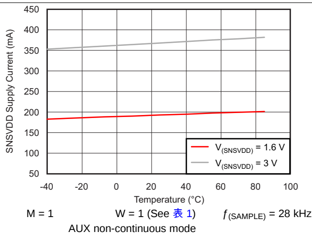
图 5. SNSVDD Supply Current vs Temperature
