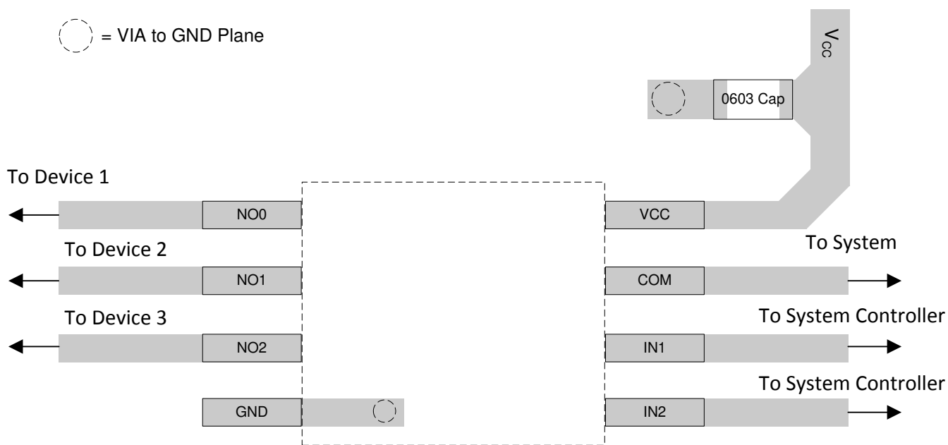
图 11-1. Recommended Layout
