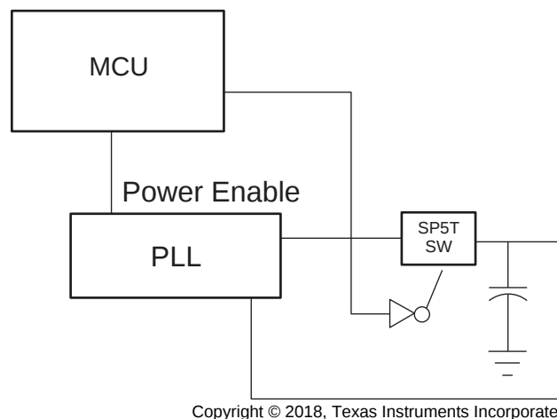
图 23. PLL Improved Power Consumption Simplified Block Diagram
