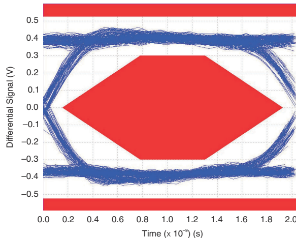
图 8-3. Eye Pattern: 480Mbps USB Signal With Switch NC Path
