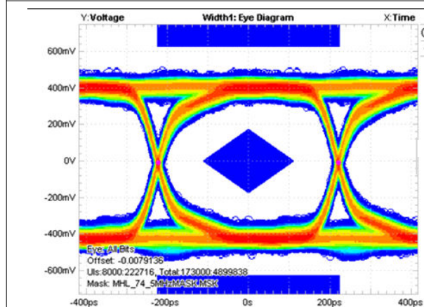
图 7-4. Eye Pattern Error Histogram: 2.25 Gbps With TS3USB3031 (Added Jitter = 5.04 ps)
