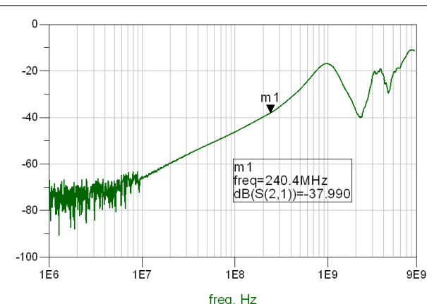
图 5-6. OFF Isolation vs Frequency for USB Path
