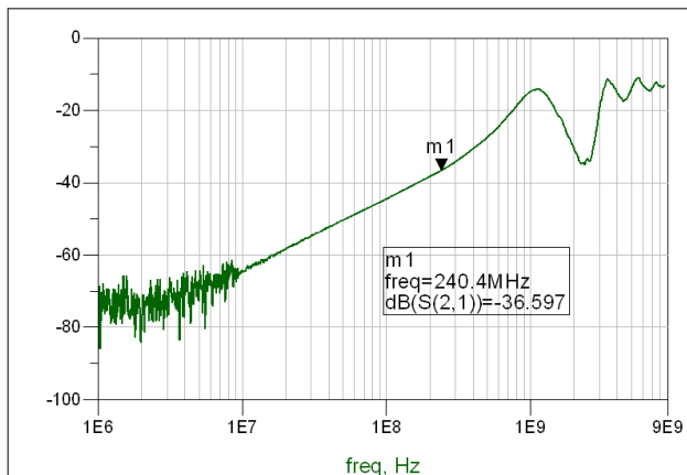
图 5-5. OFF Isolation vs Frequency for MHL Path
