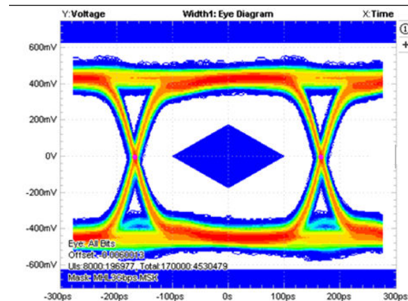
图 7-6. Eye Pattern Error Histogram: 3.0 Gbps With No Device
