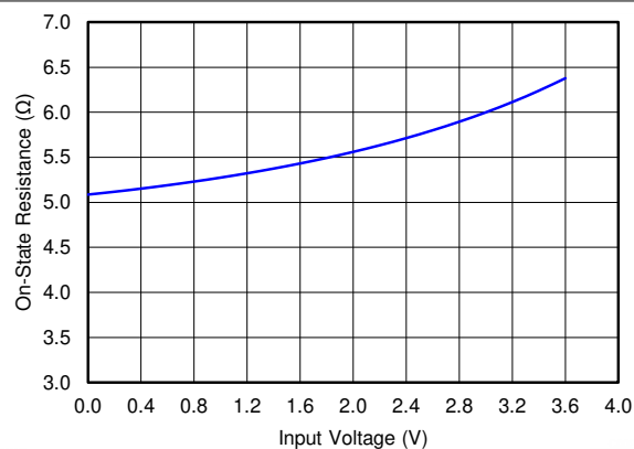
图 5-2. ON-Resistance vs V_{I/O} for USB Switch
