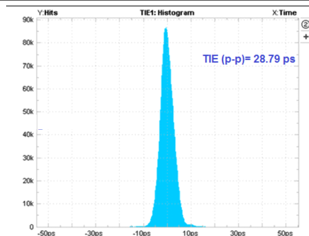
图 7-11. Time Interval Error Histogram: 4.5 Gbps With No Device
