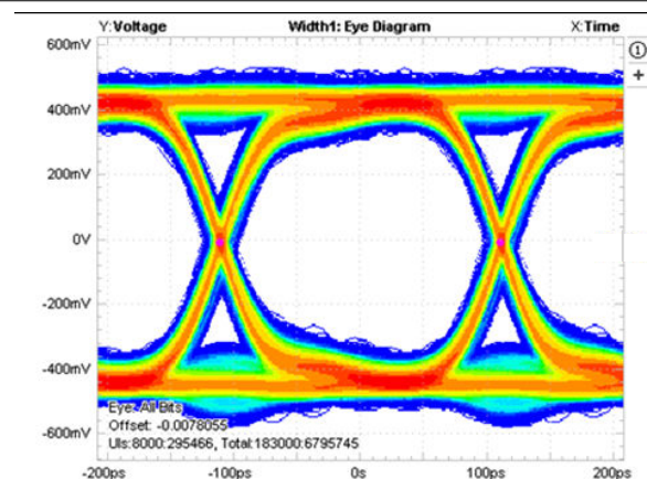
图 7-10. Eye Pattern Error Histogram: 4.5 Gbps With No Device
