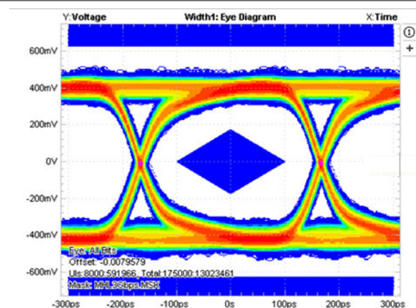
图 7-8. Eye Pattern Error Histogram: 3.0 Gbps With TS3USB3031 (Added Jitter = 2.57 ps)
