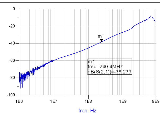
图 5-8. Cross Talk vs Frequency for USB Path
