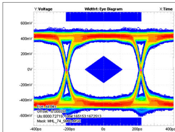
图 7-2. Eye Pattern Error Histogram: 2.25 Gbps With No Device
