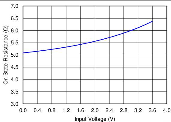
图 5-1. ON-Resistance vs V_{I/O} for MHL Switch
