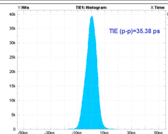
图 7-5. Time Interval Error Histogram: 2.25 Gbps With TS3USB3031 (Added Jitter = 5.04 ps)
