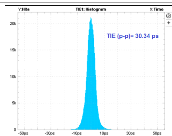
图 7-3. Time Interval Error Histogram: 2.25 Gbps With No Device
