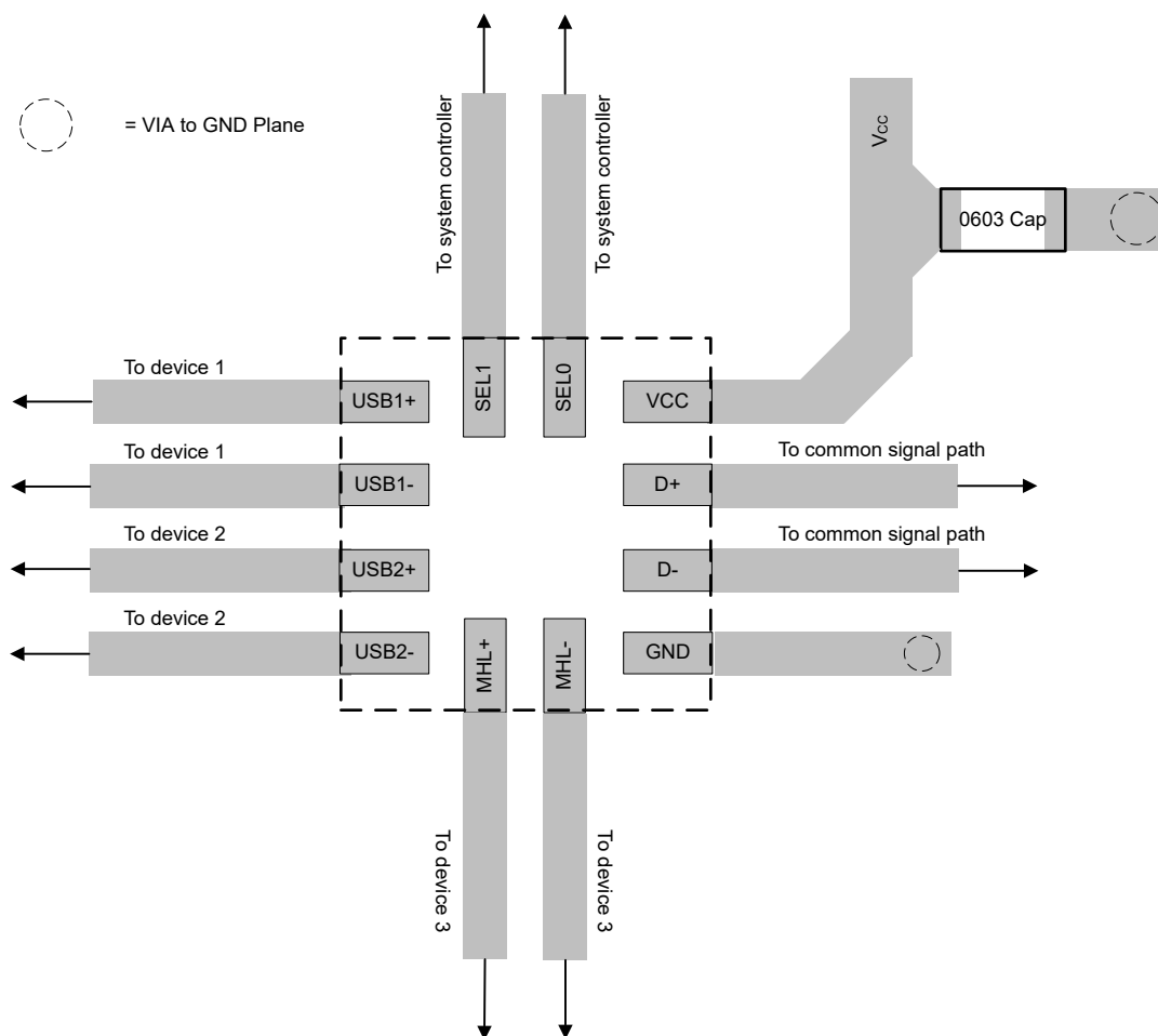
图 7-16. Layout Recommendation
