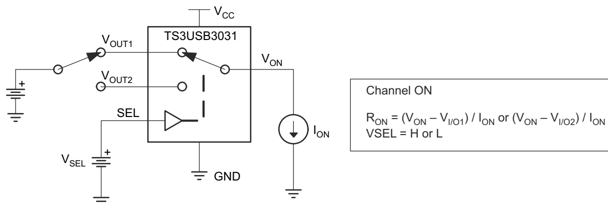
图 6-1. ON-State Resistance ( R_{ON} )
