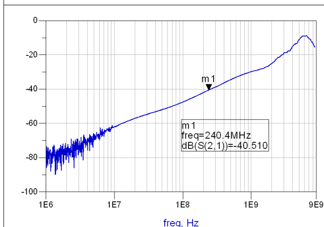
图 5-7. Cross Talk vs Frequency for MHL Path
