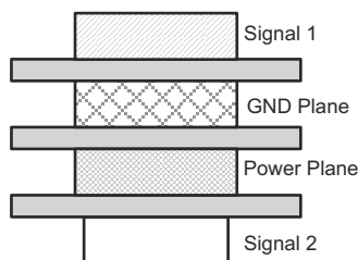
图 8-5. Four-Layer Board Stack-Up
