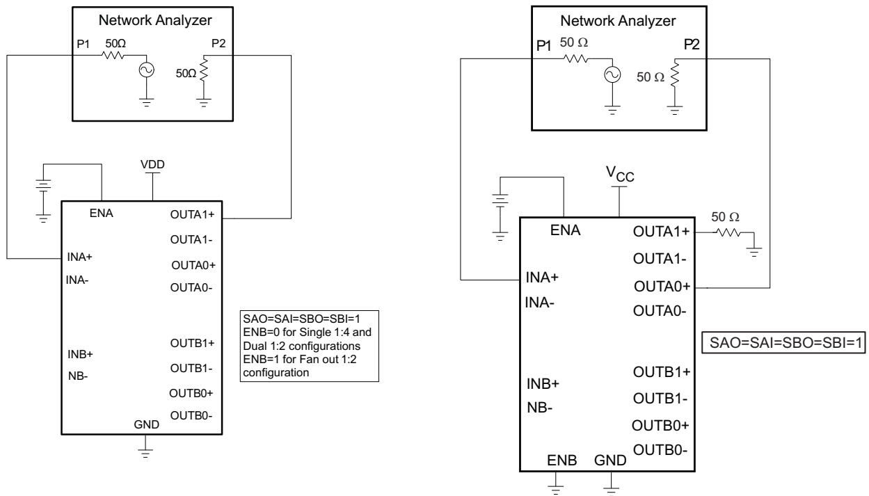
Figure 12. Off Isolation ( O_{ISO} )
