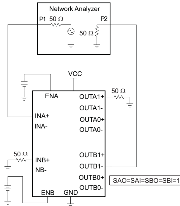
Figure 12. Off Isolation ( O_{ISO} )
