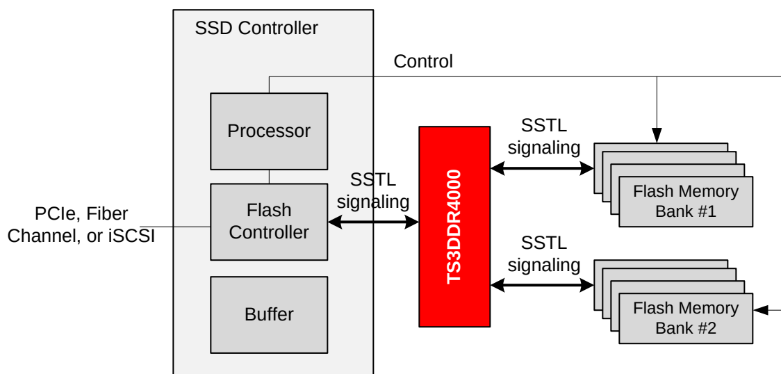
图 20. TS3DDR4000 Used In Load Isolation Application
