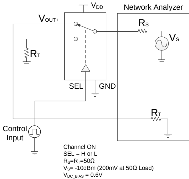
图 17. Bandwidth Measurement
