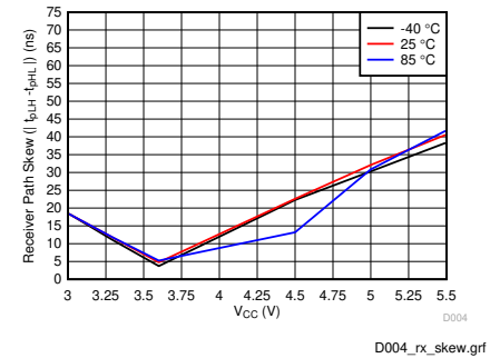
图 5-4. Receiver Pulse Skew ( t_{\text{PLH}} - t_{\text{PHL}} ) vs T_A and Supply Voltage (RGT Package)
