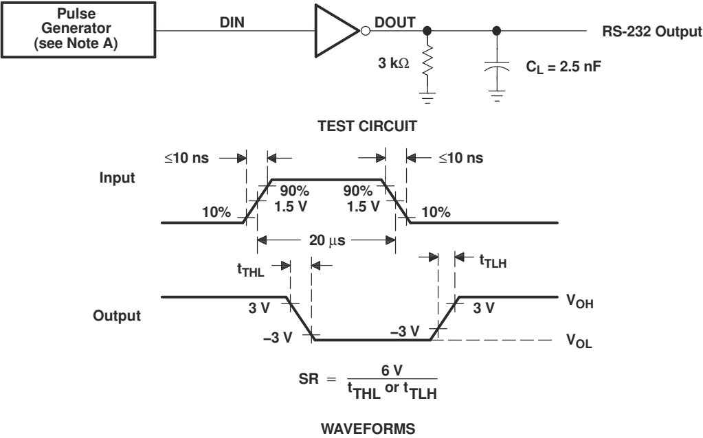
图 6-3. Test Circuit and Waveforms for t_{THL} and t_{TLH} Measurements (20 \mu s Input)
