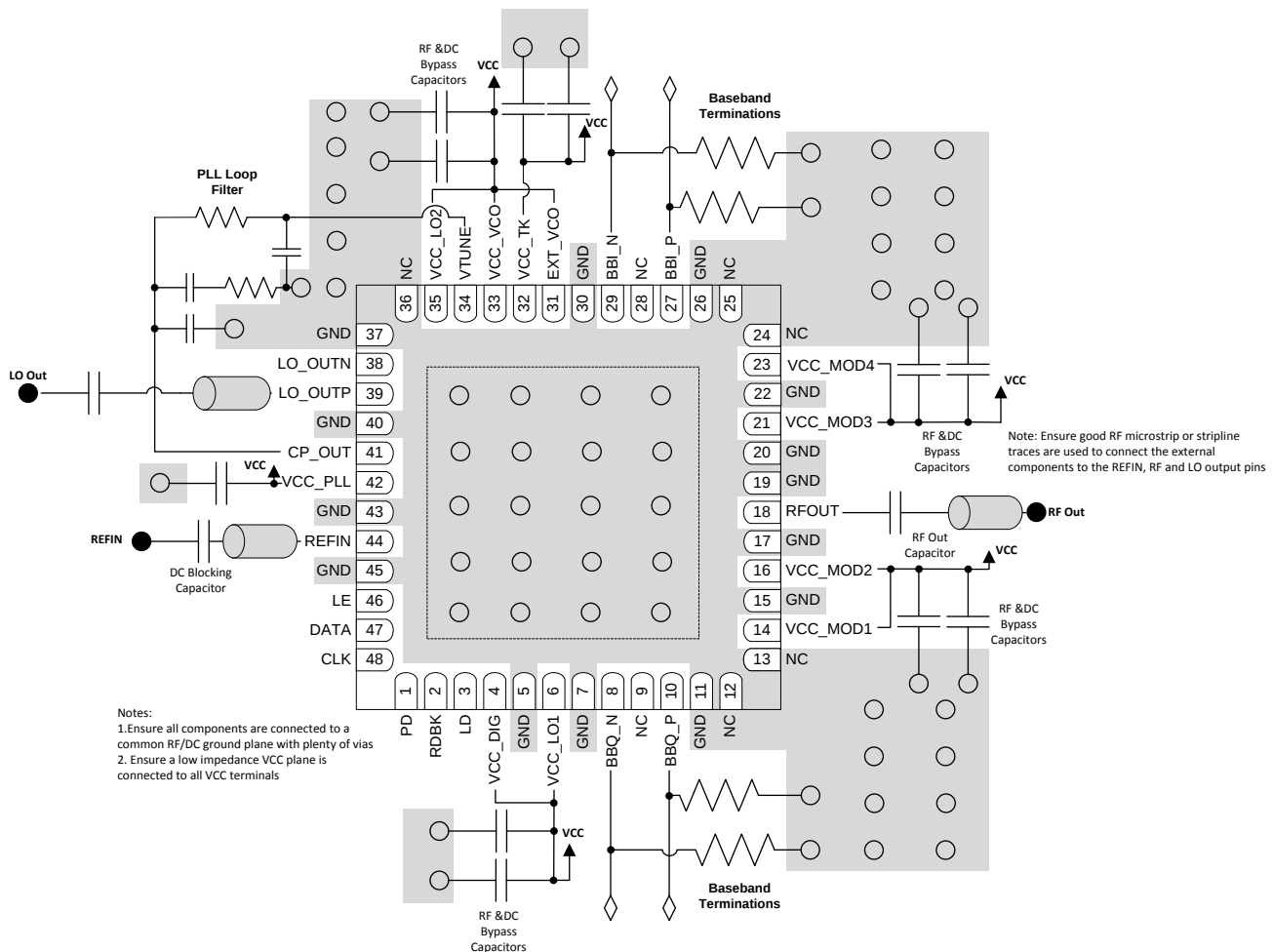
Figure 139. Layout
