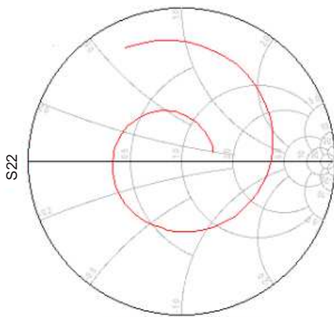
Figure 74. Smith Chart
