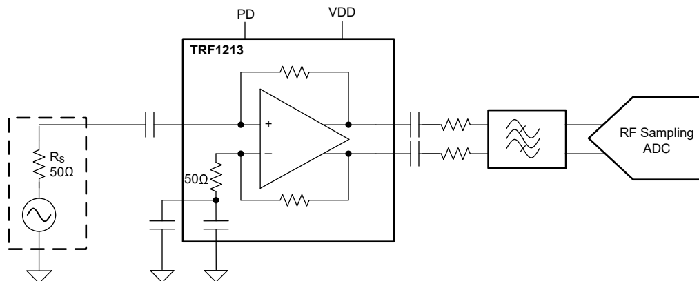
TRF1213 驱动射频采样 ADC
