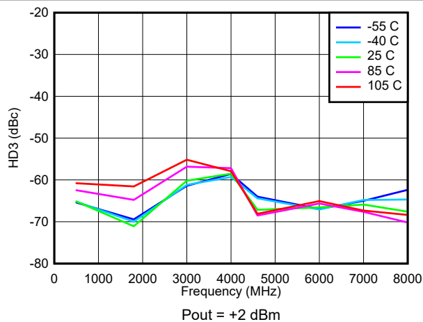
图 6-17. HD3 Across Temperature
