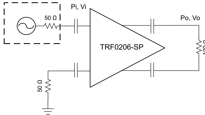
图 8-2. Power and Voltage Levels
