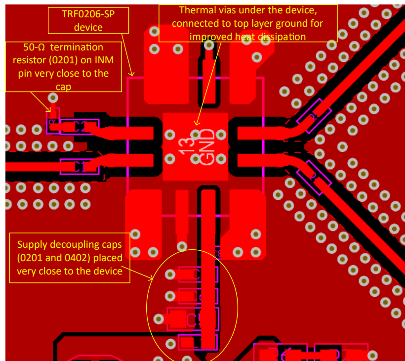
图 8-4. Layout Example: Placement and Top Layer Layout
