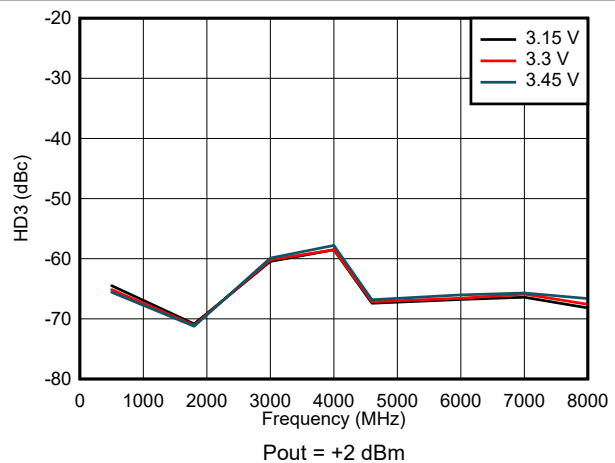
图 6-18. HD3 Across VDD
