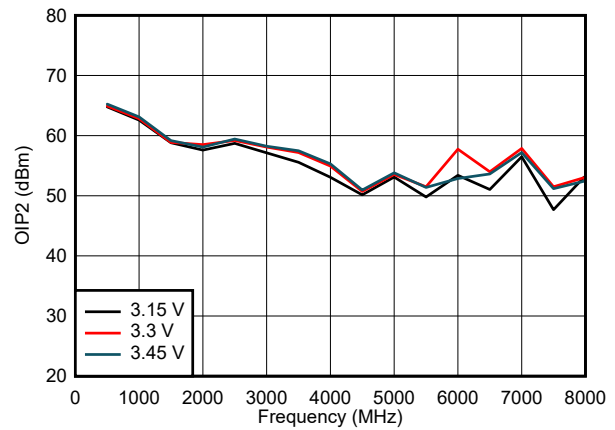
图 6-14. OIP2 Higher Frequency Across VDD
