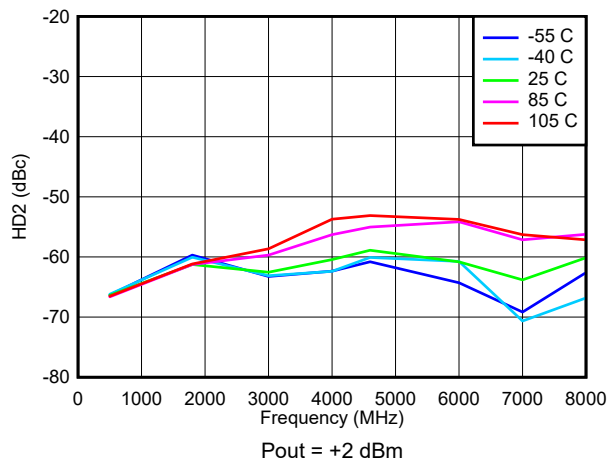
图 6-15. HD2 Across Temperature
