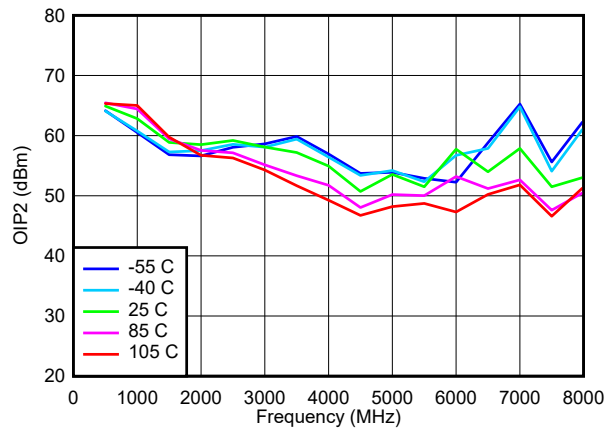
图 6-13. OIP2 Higher Frequency Across Temperature
